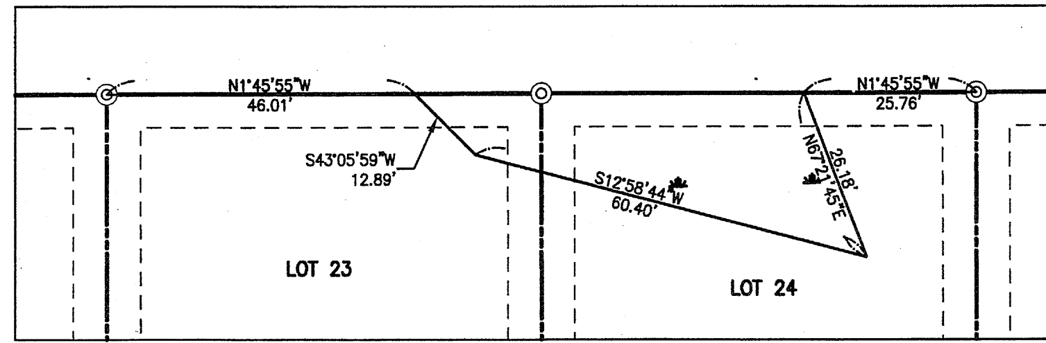
WETLAND DETAIL "B"
